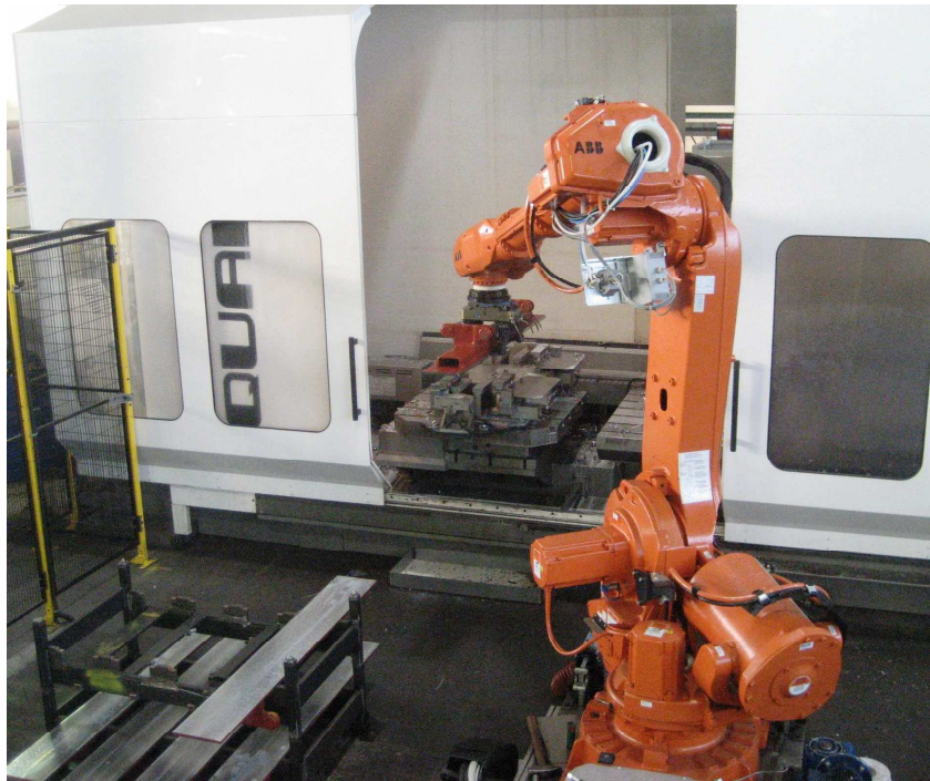
CNC Machine Center: Manufacturing of Double Belt Conveyor Metal Slats
