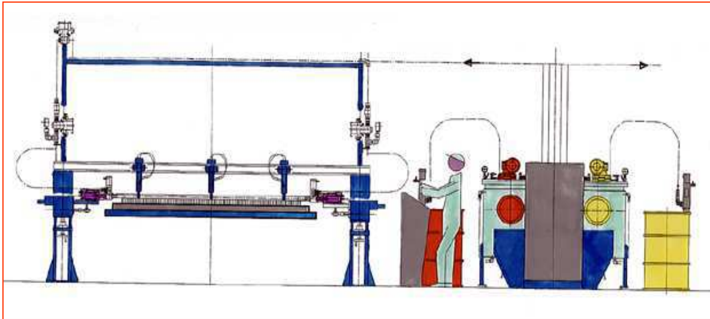
Lay-out of a discontinuous panel production plant for Truck Trailers
