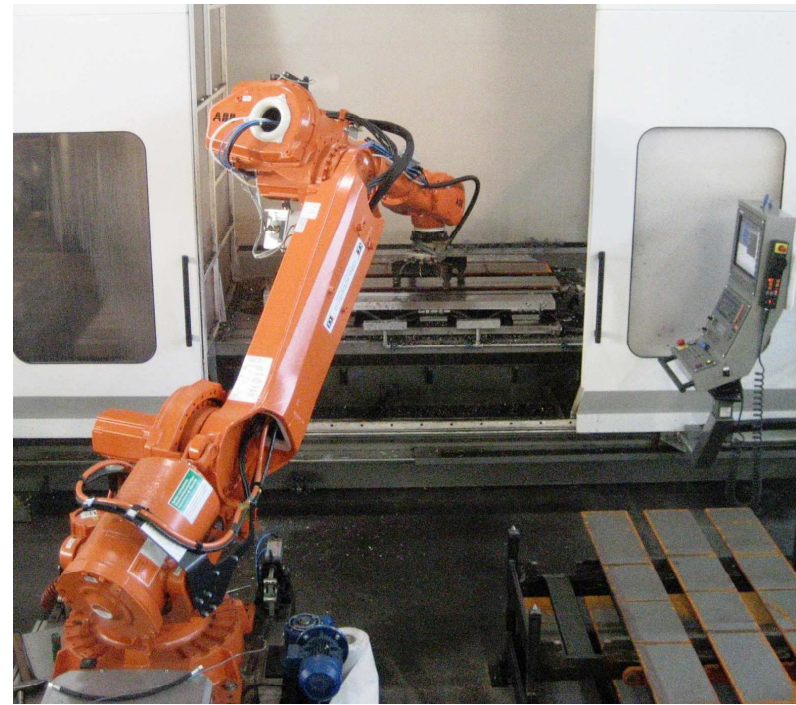
CNC Machine Center: Manufacturing of Double Belt Conveyor Metal Slats
